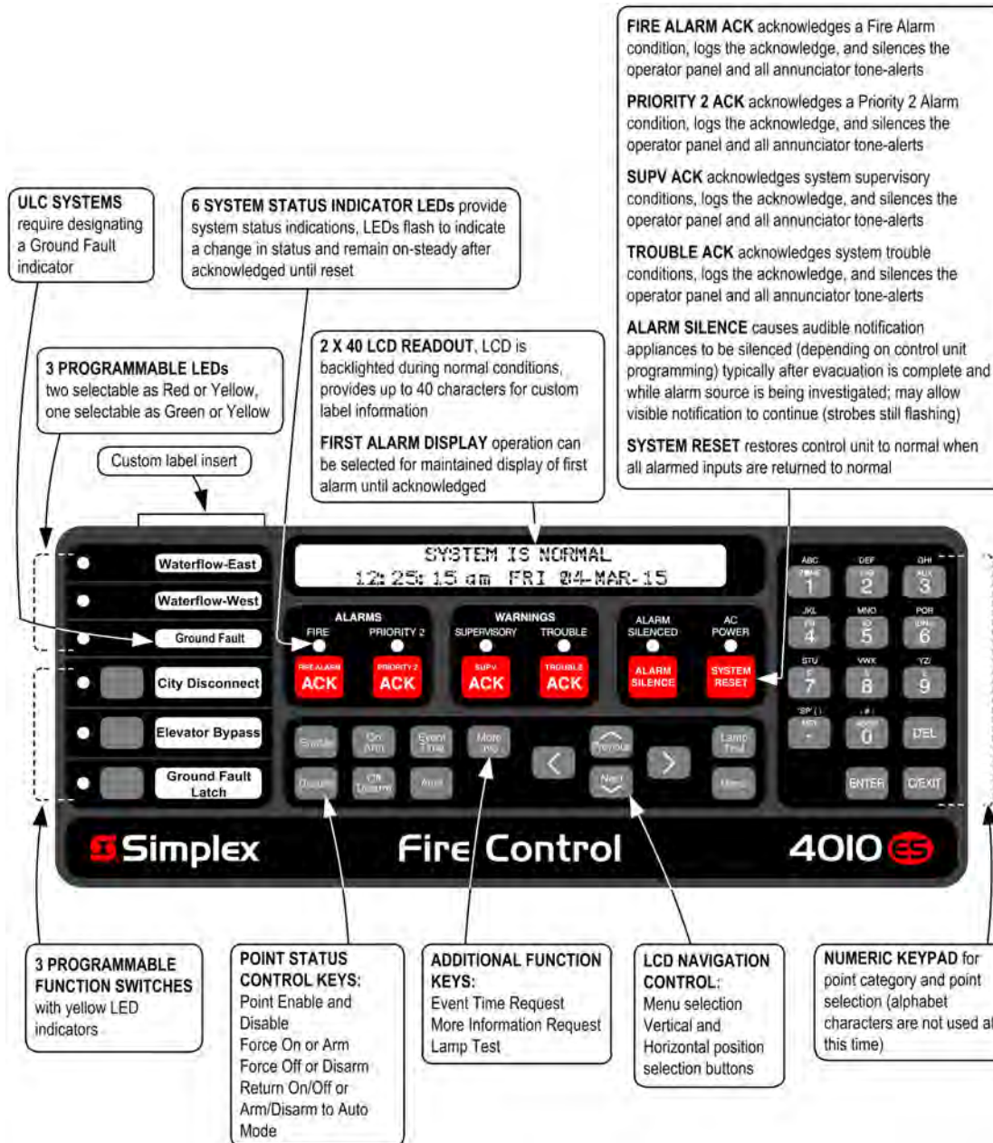
Figure 13: Operator Interface Features
