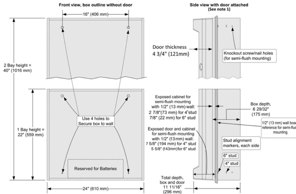
Figure 15: Cabinet dimension reference
